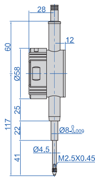
2508-25PWL/2509-25PWL
