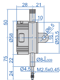
2508-10WL/2509-10WL
